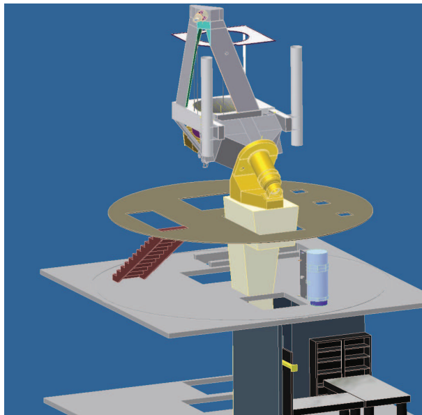
Figure 5: A cutaway sketch of CIRS location with respect to NST and Coudé Lab. The CIRS volume is represented by the blue cylinder and is located on the concrete floor above the lab.
