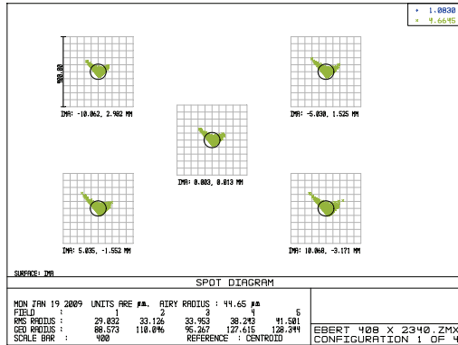
Figure 8: Spot diagram for CIRS showing performance at 1.0 and 4.6 \mu\text{m} .
