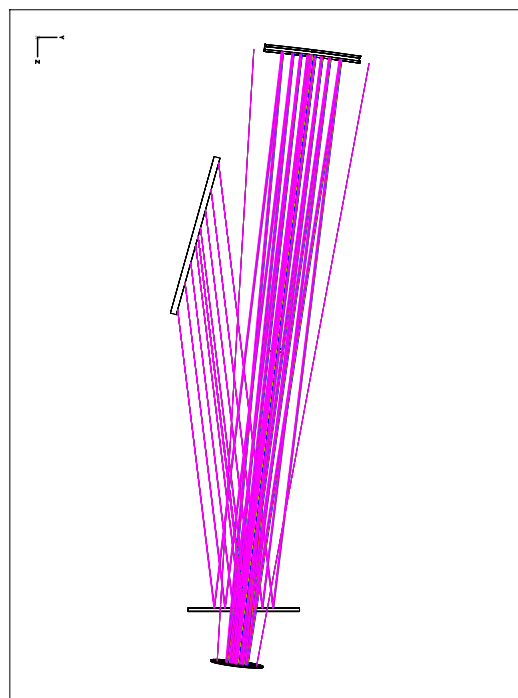
Figure 6: Schematic of the CIRS optical path. The light path is folded twice on either side of the grating to reduce the length of the instrument. The custom size grating allows the light to pass by.
