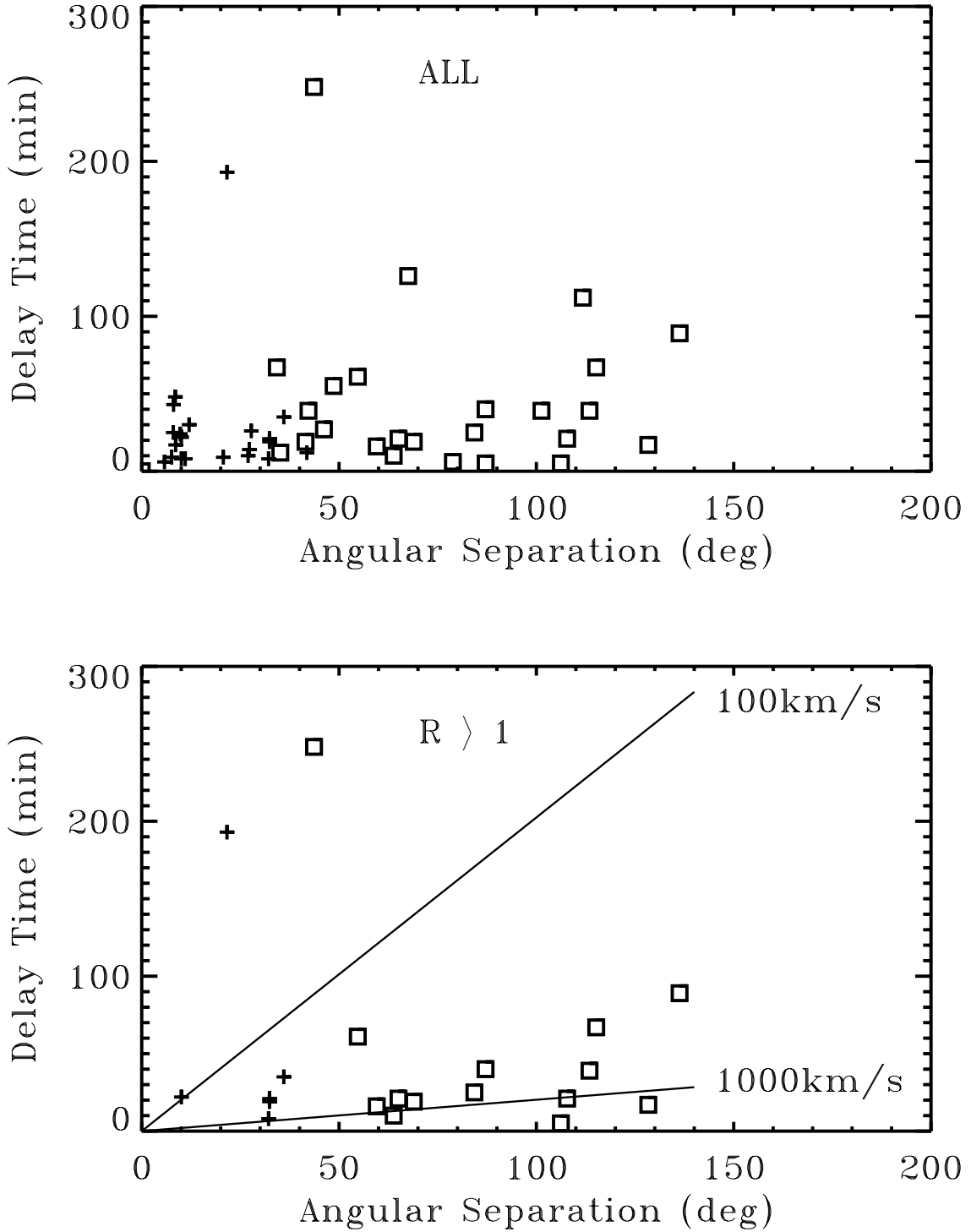
Fig. 4.— The delay time between two simultaneous flares versus their angular separation. The upper panel is for the whole data set and the lower panel is for the data subset with R > 1 . The symbols are the same as in Fig. 3. In the lower panel, two solid lines correspond to information propagation speeds of 100 \text{ km s}^{-1} and 1000 \text{ km s}^{-1} , respectively,
