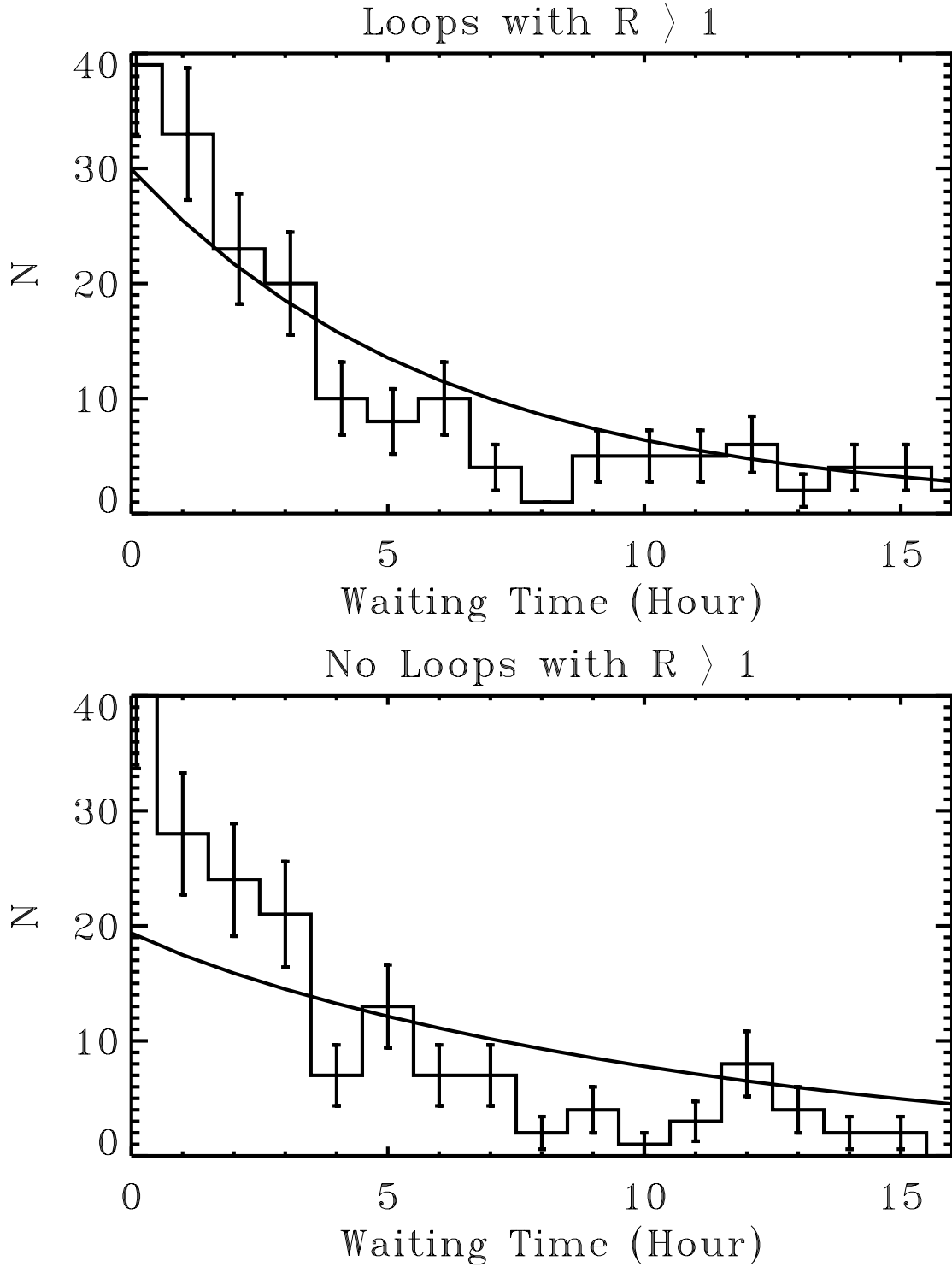
Fig. 2.— Waiting time distributions for two different subgroups of the group with R > 1 : one with loop connections (upper panel) and the other without loops (lower panel). The solid lines represent corresponding nonstationary Poisson distribution and the error bars represent the square root of the number of waiting times in each bin.
