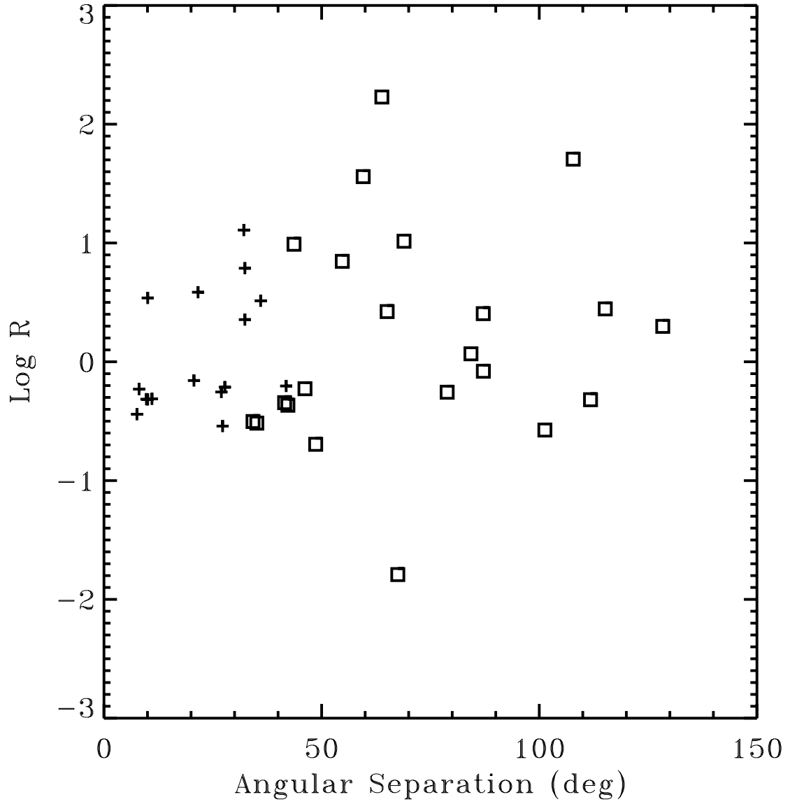
Fig. 3.— The log R of actual flaring overlap time to random-coincidence overlap time as a function of angular separation between two active regions for 38 data sets. Crosses represent simultaneous flares with SXT loop connections and squares without SXT loop connections.
