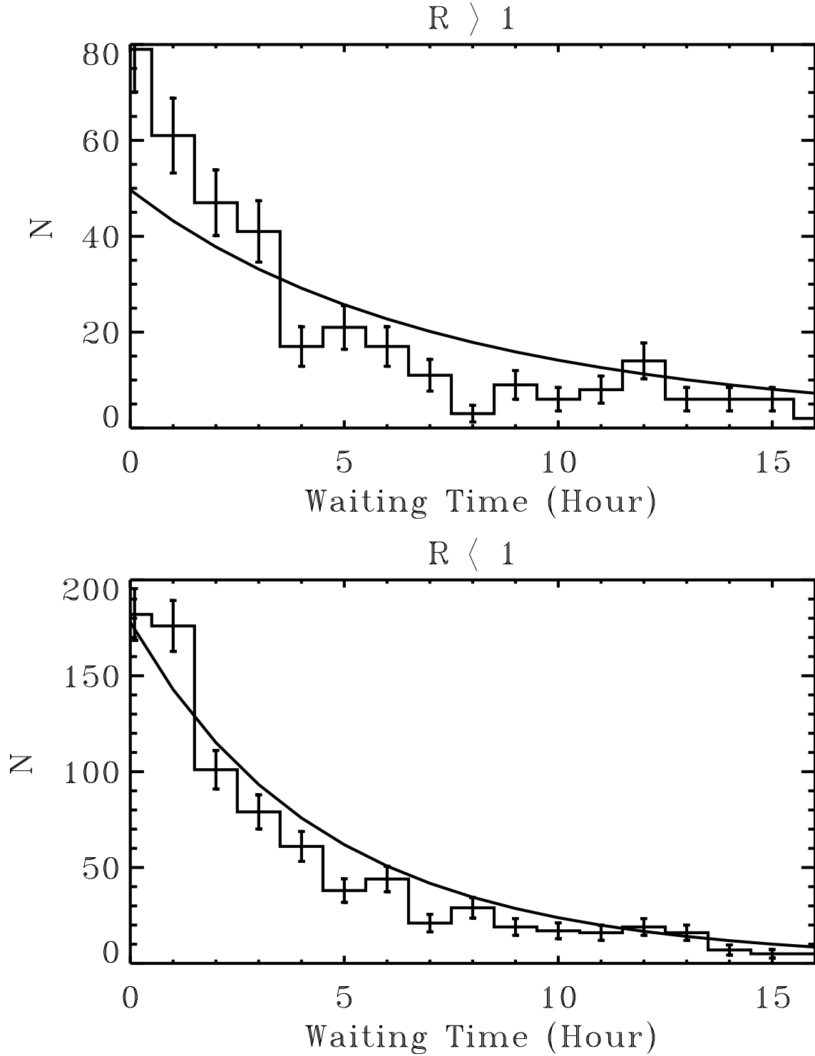
Fig. 1.— Waiting time distributions for two different groups of active region pairs which produced simultaneously flares: one with R > 1 (upper panel) and the other with R < 1 (lower panel). The solid lines represent corresponding nonstationary Poisson distributions and the error bars represent the square root of the number of waiting times in each bin.
