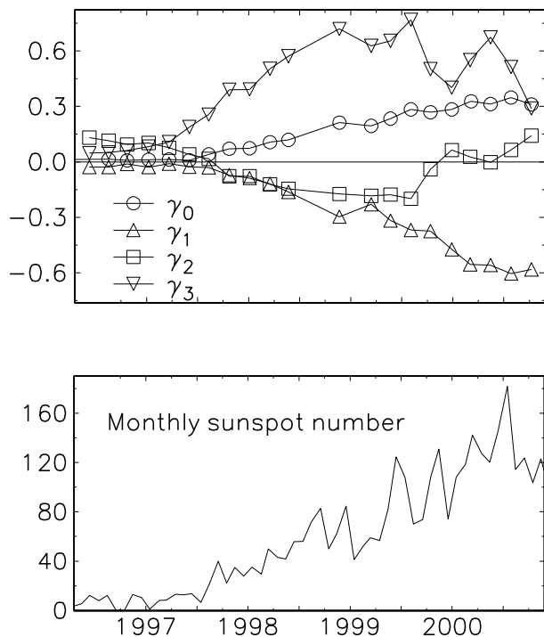
Figure 4. In the top panel, the behavior of \gamma_0 is shown as a function of time from the SOHO/MDI data, \gamma_0 is defined with respect to the 1996 activity minimum. The lower panel shows the corresponding sunspot number, which tracks \gamma_0 closely. Also, shown in the upper panel is the evolution of \gamma_1 through \gamma_3 – the P_2 , P_4 and P_6 shape asymmetries, which are generally much larger than that for P_0 .
