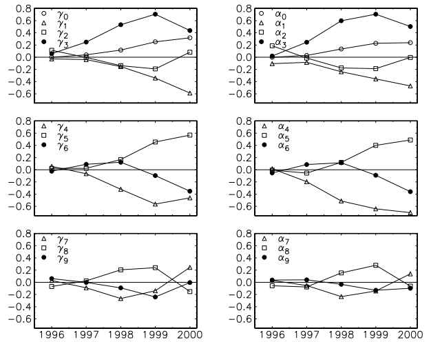
Figure 7. Right panels show the Legendre polynomial expansion of the photometric signal following the analysis in Goode et al. (2001). Left panels show the corresponding \gamma 's. The latter were averaged to the time frame of the \alpha 's.
