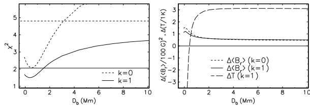
Figure 6. Left panel shows the \chi^2 from fitting \gamma_0 and \gamma_1 to Eqs.(8) and (9) with B_r given by Eq.(10) with D_b treated as the adjustable parameter. Flat dashed and solid lines are for constant \gamma 's. Right panel shows the implied field intensity and the temperature change.
