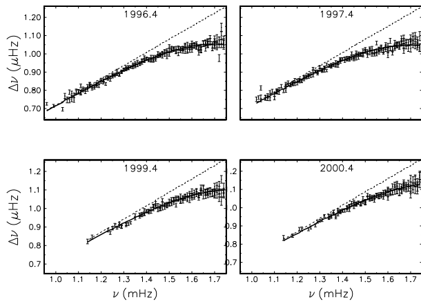
Figure 1. Differences between measured and calculated f-mode frequencies. The error bars show estimated standard deviations of measured values. The dates correspond to the center of the individual 72-day long measurement periods. The solar model was calculated assuming R_{\odot} = 695.991 Mm. The solid line represents the fit to Eq. (4). The dashed straight line represents the part attributed to the difference between the solar radius and that adopted in the model.
