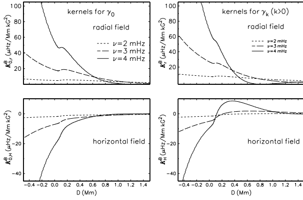
Figure 5. Kernels for the \gamma 's at three selected frequencies plotted as functions of the depth in outer part of the standard solar models.
