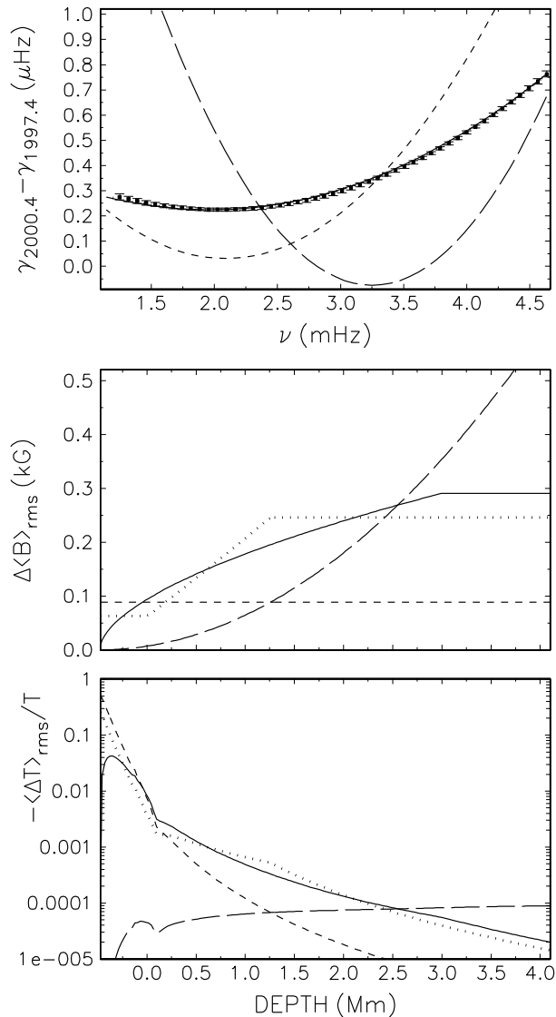
Figure 3. In the top panel, points with the error bars represent \Delta\gamma_0(\nu) inferred from p-mode frequency difference between 2000.4 and 1997.4. The lines correspond to various distributions of the averaged magnetic field, shown in the middle panel. The solid and dotted lines are within the error bars in the top panel. The bottom panel shows the relative temperature decreases required to cause similar frequency shifts as the corresponding magnetic field increases.
