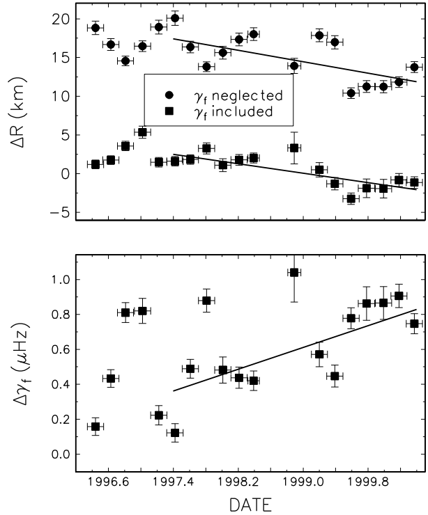
Figure 2. Upper panel: Variation of solar radius between 1996.4 and 2000.4 inferred from f-mode frequencies with and without the \gamma_f -term. Two straight lines represent linear fits to the data starting from 1997.4 when the rise of cycle 23 began. Lower panel: Corresponding variation of \gamma_f , which describes remaining near-surface contribution to f-mode frequency variations.
