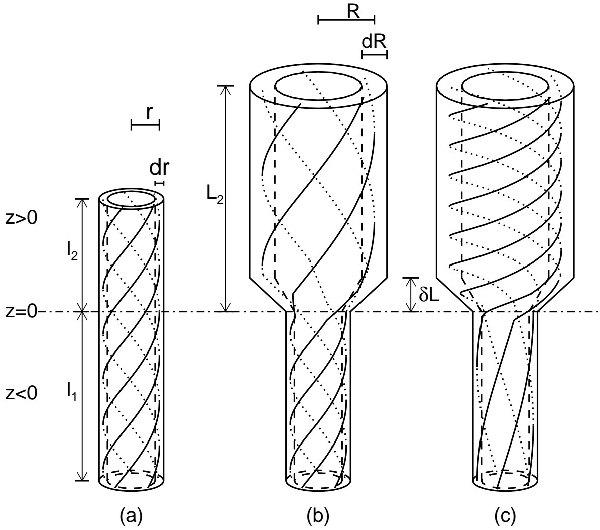
Fig. 3.— Helicity transfer by the expansion of the coronal segment of a twisted flux tube: (a) initial flux tube, (b) expansion conserving the helicity on each segment, and (c) expansion keeping the torque balanced between the two segments.
