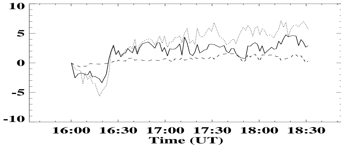
Fig. 2. — Temporal change of the weighted mean shear angle relative to the initial shear angle for the boxed area in Figure 1. The dotted line is what Wang et al.(2002) obtained using the potential method for the 180^\circ ambiguity and the solid line is what we obtained from the present study. The dashed line corresponds to the temporal variation of weighted potential field, the last term of equation (8).
