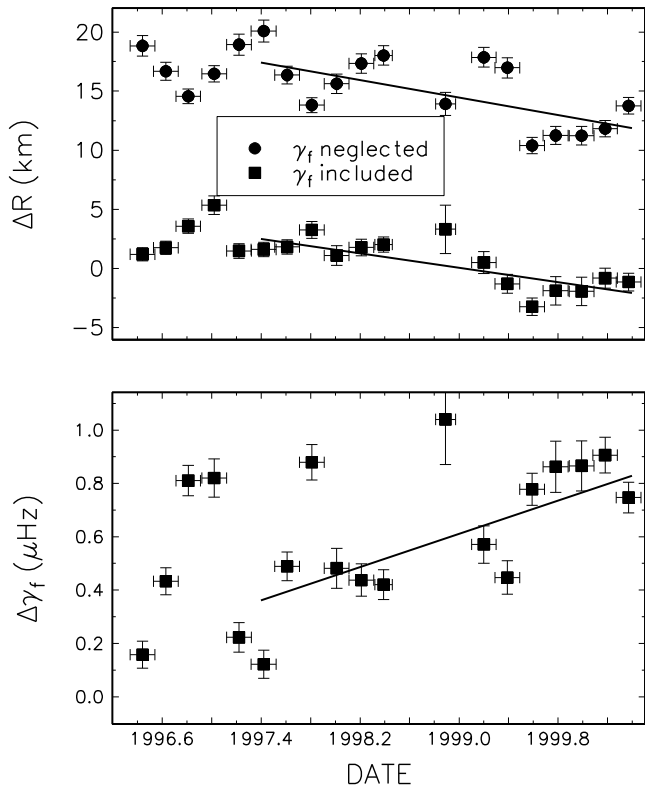
Fig. 2. — Upper panel: Variation of solar radius between 1996.4 and 2000.4 inferred from f-mode frequencies with and without the \gamma_f -term. Two straight lines represent linear fits to the data starting from 1997.4 when the rise of cycle 23 began. Lower panel: Corresponding variation of \gamma_f , which describes remaining near-surface contribution to f-mode frequency variations.
