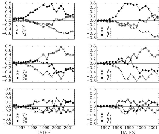
Fig. 4. — In the left panels, the behavior of \gamma_k ( k > 0 ) is shown as a function of time from the SOHO/MDI data. The right panels show the corresponding \beta 's. It is clear that there is detailed agreement to P_{18} (or \gamma_9 ), which bears out the close relation of what happens just beneath the surface to what happens in the atmosphere.
