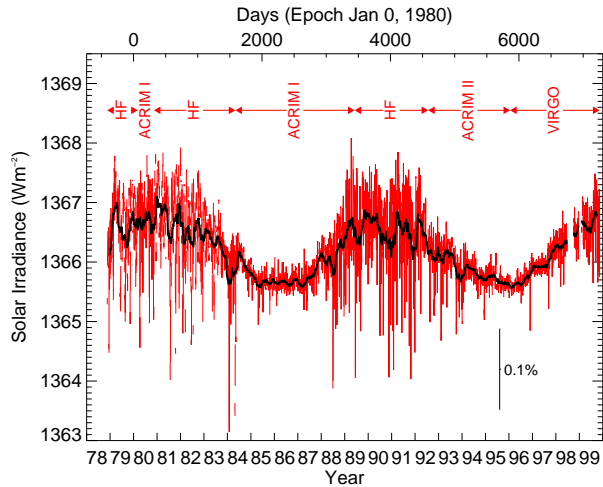
Fig. 1. — Measured solar irradiance (in watts per \text{m}^2 ) vs. time (Fröhlich 2000)
