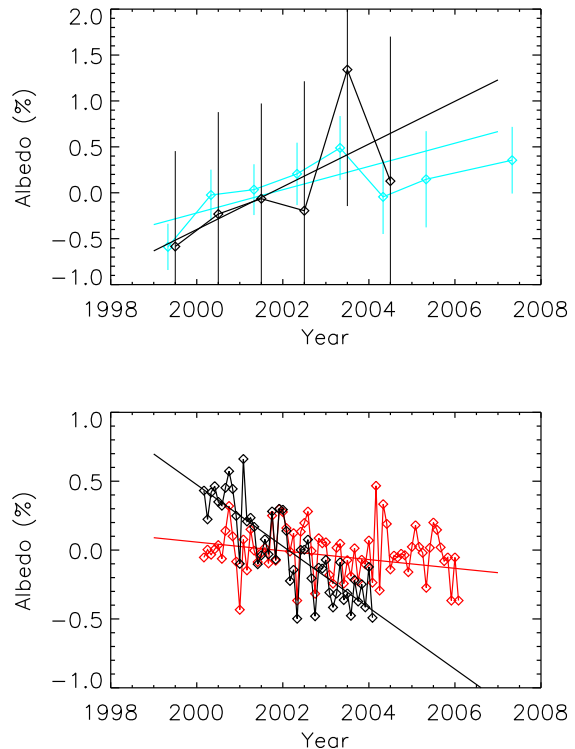
Figure 2: Top: Inter-annual Earth albedo anomalies as measured by earthshine. In black are the albedo anomalies published in 2004, following Palle et al. (2004), and in blue are the updated albedo anomalies after our improved data analysis, which also included more years of data. Bottom: Inter-annual Earth albedo anomalies as measured by CERES. In black are the albedo anomalies published in 2005, following Wielicki et al. (2005), and in red are the updated albedo anomalies after their improved re-calibration of the on-board sensors (Loeb et al., 2007). To evaluate the recalibration effects, a linear fit is applied to both datasets within each panel using only the data over the common period of 2000-2004. For both, Earthshine and CERES, the linear fit to the full dataset up to 2006 would not differ much.
