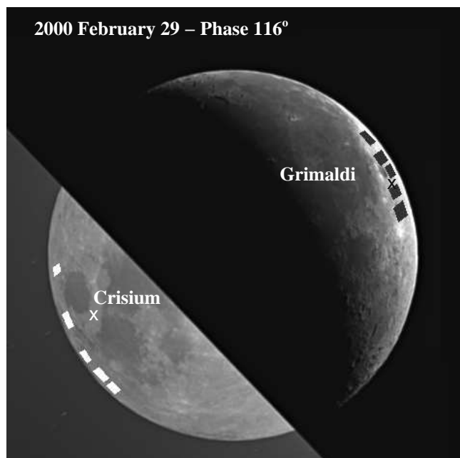
Figure 1. The moon showing the bright side and the earthshine. The Grimaldi side is in the moonshine (brightside) and the Crisium side is in the earthshine. Our ten highlands fiducial patches used in the observations made from BBSO are indicated. The crosses give the approximate positions of Danjon’s (1928,1954) fiducial patches. Goode et al. (2001) used one fiducial patch on each side, and on the Crisium side it is the one closest to the white cross, while on the Grimaldi side, it is the one immediately above the black cross. In the image, the lunar phase is 115^{\circ}.9 , near a declining quarter moon. Unlike the moonshine, the earthshine is flat across the disk. The flatness is due to the uniform, incoherent back-scattering (non-Lambertian), in contrast to the forward scattering of sunlight occurring in the sunlit lunar crescent surface.
