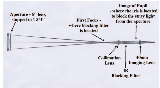
Figure 3. Schematic of the earthshine telescope optical train. At prime focus during the earthshine exposures, the moonshine blocker translates and rotates to its proper position to shield out the brightside. At the image of the pupil, the edges of the entrance aperture are blocked to reduce stray light. The earthshine camera chip is at the second focus.
