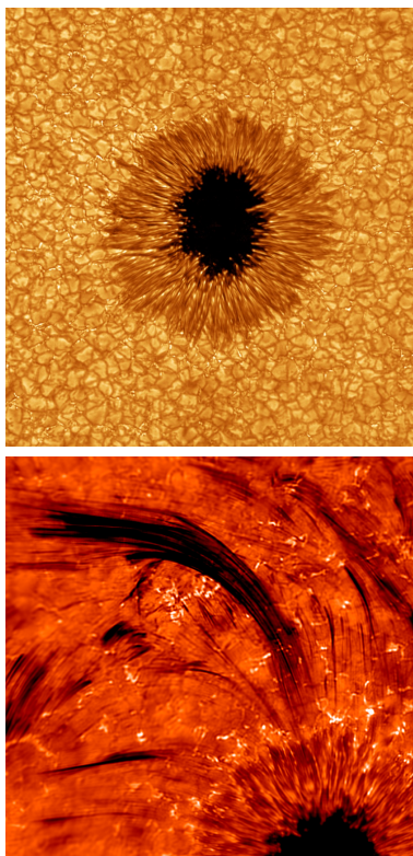
Figure 2. Top: A small sunspot observed on 2 July 2010. Bottom: H \alpha image of the same sunspot revealing the dynamical layer overlying the surface region shown in the full sunspot image. Most apparent are the long dark streaks, so-called “jets” arising from the bright magnetic regions on the edge of the penumbra. Both images benefited from adaptive optics, which enabled real-time correction for atmospheric distortion.
