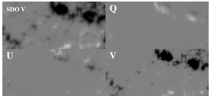
Figure 3. Top left: Stokes V image of SDO/HMI for comparison to IRIM vector magnetogram of a cluster of pores near AR 11121 at 231E 391S, taken on Nov. 09, 2010. Top right: calibrated Stokes Q image, bottom left: calibrated Stokes U image, and bottom right: calibrated Stokes V image. Dual-beam technology was employed to minimize seeing-induced noise. The center of the strongest pore has a longitudinal magnetic field strength of about 1 kG. The field of view of IRIM is about 50'' \times 25'' .
