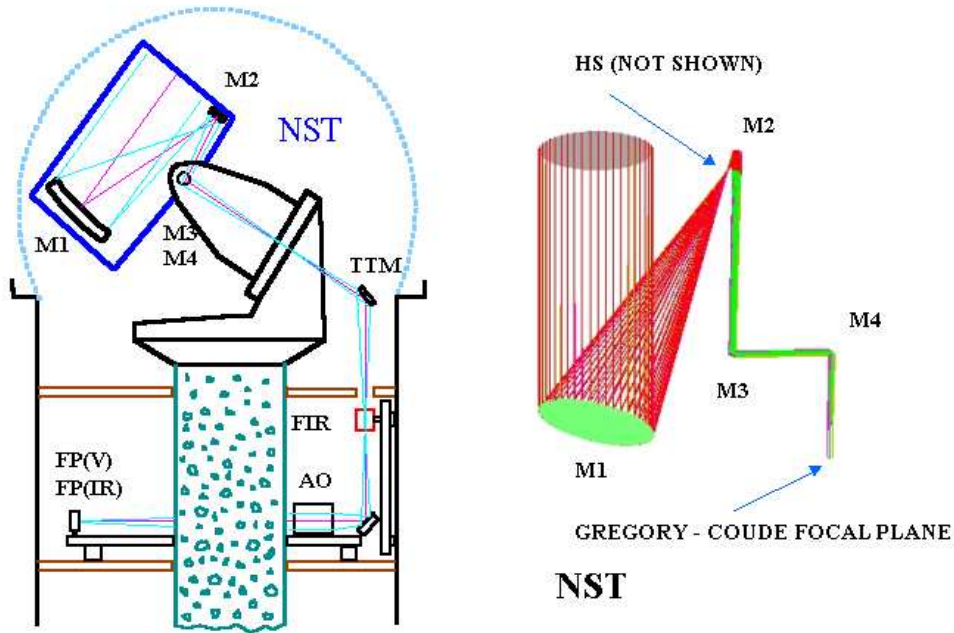
Figure 2: (Left) Schematic of the new open telescope and its retractable dome (not to scale). Typically, the light goes to the Fabry-Pérot-based scientific channels in the visible and near-IR, labelled FP(V) and FP(IR), which reside on the horizontal optical tables. The optical tables are installed on the floor beneath the telescope. Future Far-IR (FIR) instrumentation would require only a tip/tilt mirror (TTM) to get diffraction-limited images. The visible and near-IR channels would be operating downstream of the high-order AO system. We anticipate placing the polarizing optics between M2 and M3, where the light is nearly parallel. (Right) The optical layout of the NST with a true relative scale (a Zemax created model). The NST is an off-axis section of a conventional Gregory telescope with parabolic primary mirror M1, elliptical secondary M2, removable (for access to the primary focal plane with a wide FOV) heat-stop mirror HS, flat folding mirrors M3 and M4 (coudé mirror). M3 is a fixed folding mirror. The off-axis primary has an f-ratio 2.4 (parent's f-ratio is about 0.73). The telescope's effective focal length is about 80 m with a final f-ratio of 50, which is close to that of the current 65 cm telescope. The image scale in the Gregory-Coudé focal plane is 2.6''/\text{mm} . TTM redirects light to the floor below to get diffraction-limited images for far-IR instrumentation.
