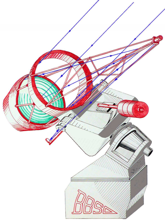
Figure 1: Schematic of the 1.6 m off-axis, open NST for which the primary mirror is as close to the declination axis as possible. The optical path is indicated. There is a Nasmyth-focus along the declination axis, where we can put instrumentation. In this design, the coudé mirror is simply a flip mirror to re-direct light from the declination axis to the floor below, where the AO and principal instrumentation reside.
