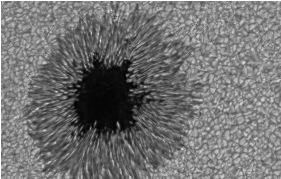
Figure 2: Speckle reconstruction of active region NOAA 8673 observed with the 1k \times 1k pixel, 12-bit SMD CCD camera on 27 August 1999. The FOV is 76'' \times 40'' , the exposure time is 4 ms, and the Fried-parameter amounts to 12.6 cm.
