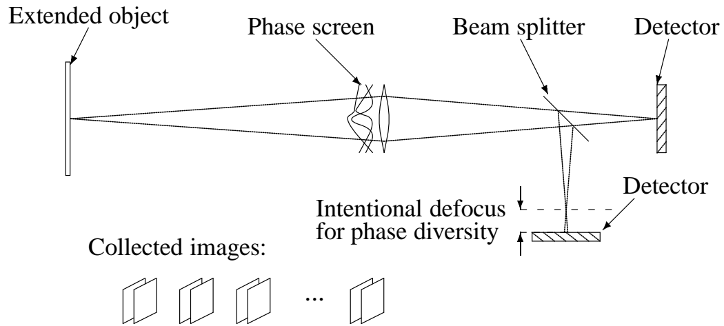
Figure 1: Typical data collection scheme, illustrating the data collection model. Only the straight through path is used for speckle interferometry. Short exposure images are collected for each of multiple atmospheric realization. For phase diversity methods, the conventional short-exposure images are supplemented with additional, simultaneous images that are intentionally defocused.
